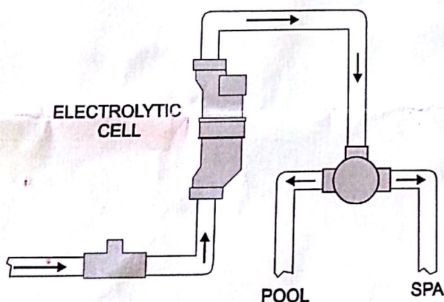
Vertical Installation
