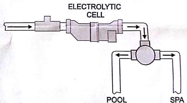
Inverted Installation
